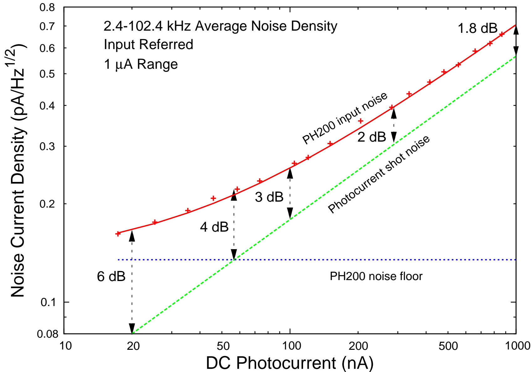
PH200 1 \mu A Range: 2-102 kHz Current Noise Vs Photocurrent
